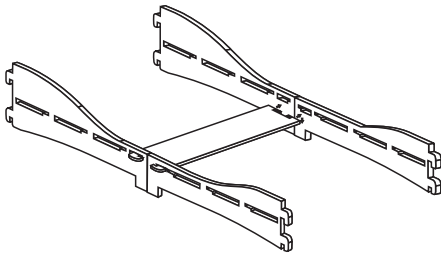
Step 1—slot central support onto side rails
